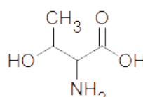
Threonin
