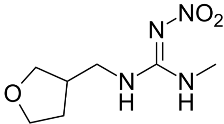
Dinetofuran
