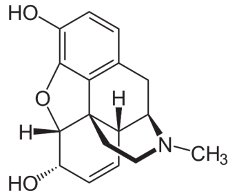
Morphin
