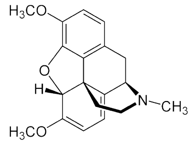
Thebain
