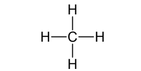
a) Methan
